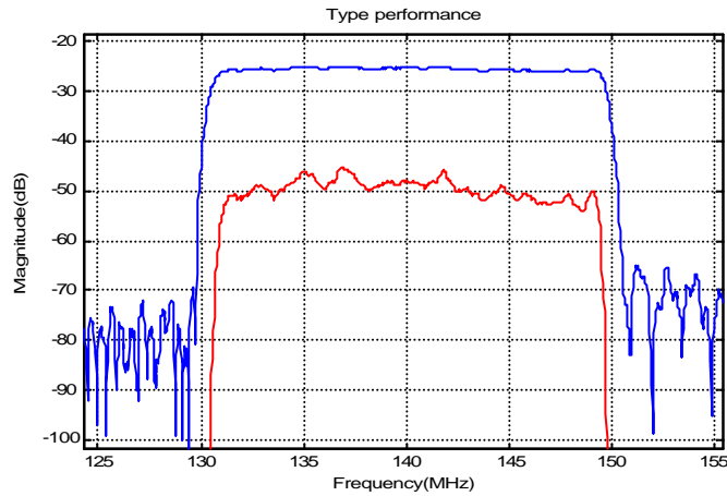
SP140B19 SAW Filter Typical Performance
